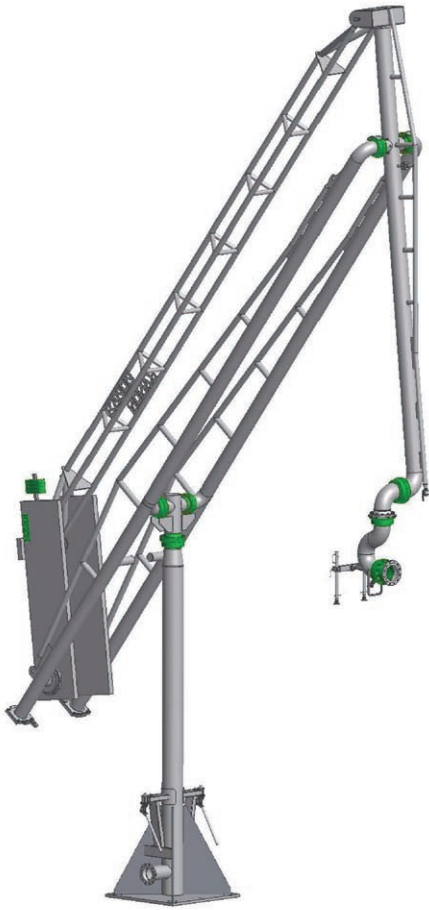
Figure 3. MLA with self supporting piping and symmetric structure.
