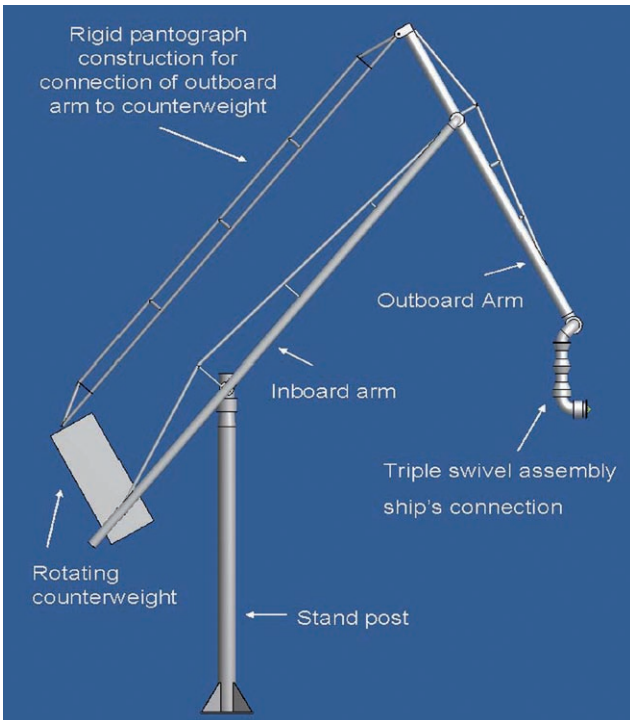
Figure 1. Basic design.
