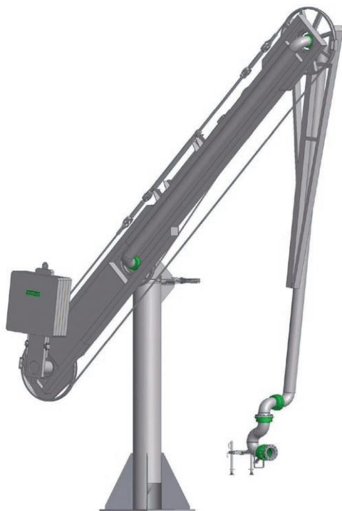
Figure 2. MLA with cable and wheel assembly and support frame.
